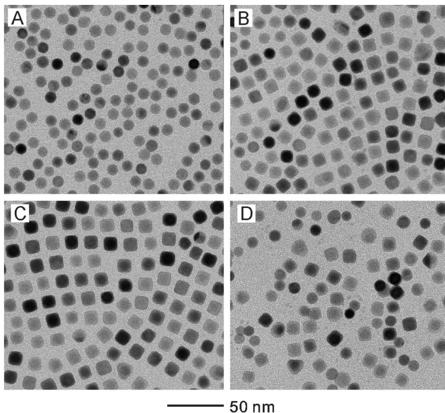
Figure 4. TEM images of the samples prepared under the same condition as in Figure 2, except the use of CTAB instead of CTAC as a capping agent during the growth of silver. After the injection of \text{AgNO}_3 and AA, the concentrations of \text{AgNO}_3 were: (A) 0.09, (B) 0.17, (C) 0.29, and (D) 0.67 mM, respectively.
