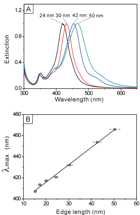
Figure 7. (A) UV-vis extinction spectra of Au@Ag core-shell nanocubes obtained under the same conditions shown in Figure 3, indicating that the main LSPR peak red-shifts with the increase in edge length. (B) A plot showing the linear dependence between the major LSPR peak position and the edge length for the Au@Ag core-shell nanocubes.
