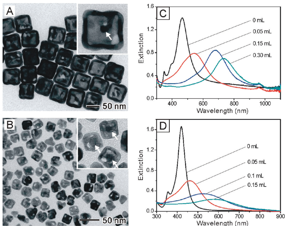
Figure 8. TEM images of Au-based nanocages derived from the Au@Ag nanocubes of (A) 50 and (B) 21 nm in edge length, respectively. The wall thicknesses of the Au nanocages were (A) 8.8 \pm 0.9 and (B) 4.2 \pm 0.4 nm, respectively. Insets show the corresponding images at higher magnification, clearly revealing the existence of the original Au seeds in the interiors (marked by white arrows). (C,D) UV-vis extinction spectra taken from aqueous suspensions of Ag nanocubes (C) 50 and (D) 21 nm, respectively, in edge length after they had been titrated with different volumes of an aqueous 0.5 mM HAuCl 4 solution (as labeled on each curve).
